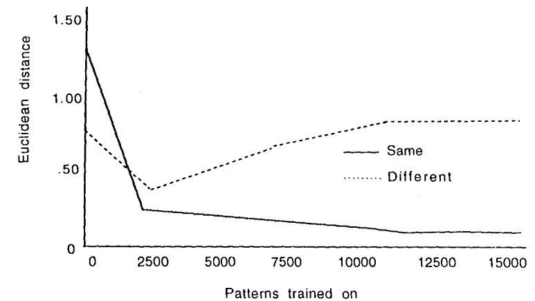
Fig. 7. The Euclidean distance between patterns of activation on the hidden layer for pairs of inputs same on the queried dimension (solid line) or different on the queried dimension (dashed line) as a function of training patterns in the Joint training regimen of simulation 2.
