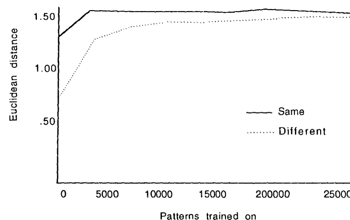
Fig. 4. The Euclidean distance between patterns of activation on the hidden layer for two input objects that are the same on the queried dimension and different on all other dimensions (solid line) and for two input objects that are different on the queried dimension and the same on the other three (dashed line) as a function of training patterns.
