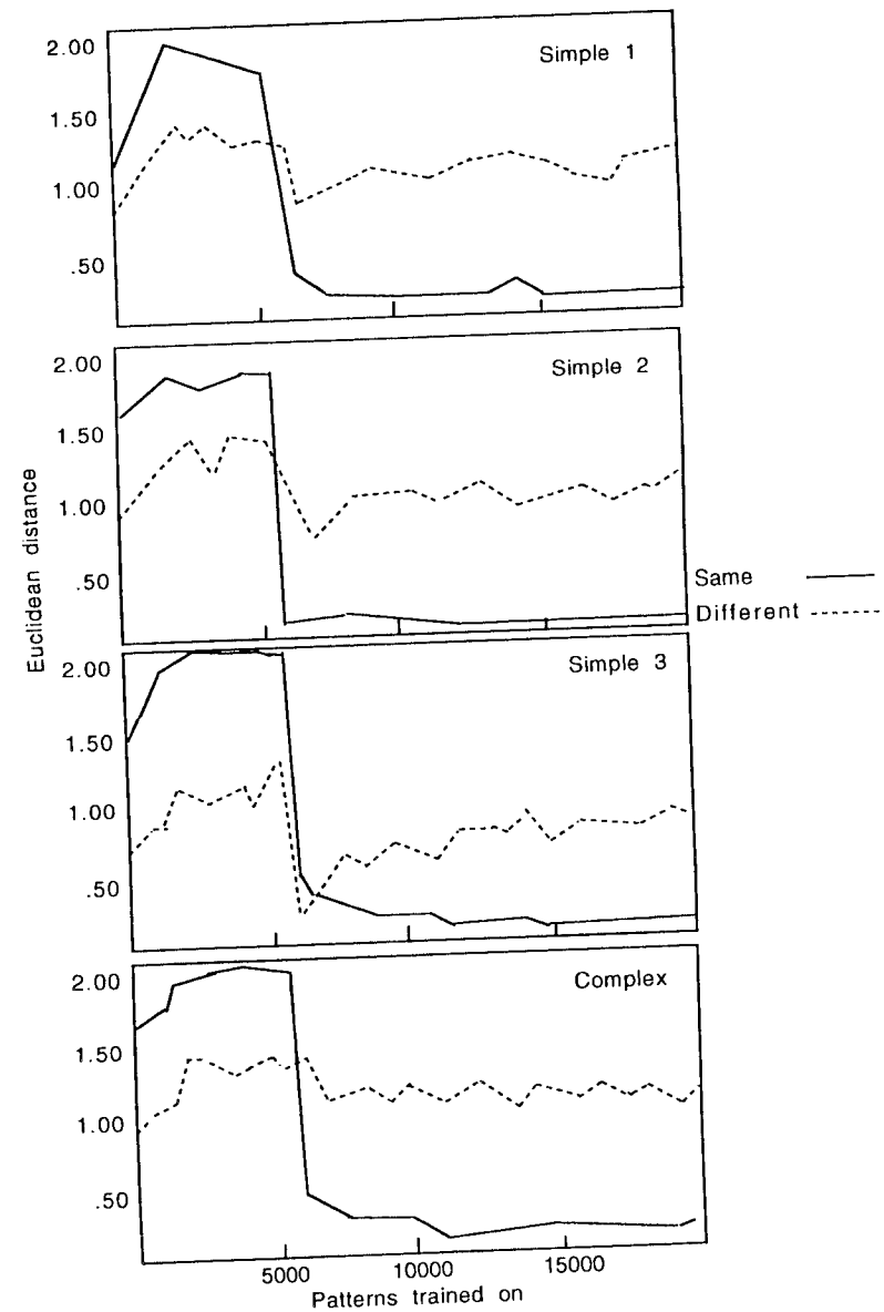
Fig. 11. The Euclidean distance between patterns of activation on the hidden layer for pairs of inputs same on the queried dimension (solid line) or different on the queried dimension (dashed line) as a function of training patterns in the Incremental training regimen of simulation 3 for the three Simple and one Complex dimensions. Comparison training introduced after 5000 trials.
