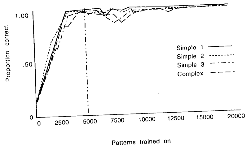
Fig. 10. Proportion correct responses in the attribute labeling condition under the Incremental training regimen for the three Simple dimensions that correspond to sensory dimensions and for the Complex dimension. Comparison training was introduced after the first 5000 trials.
